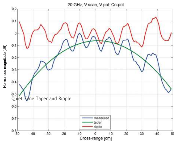
Quiet Zone Taper and Ripple
