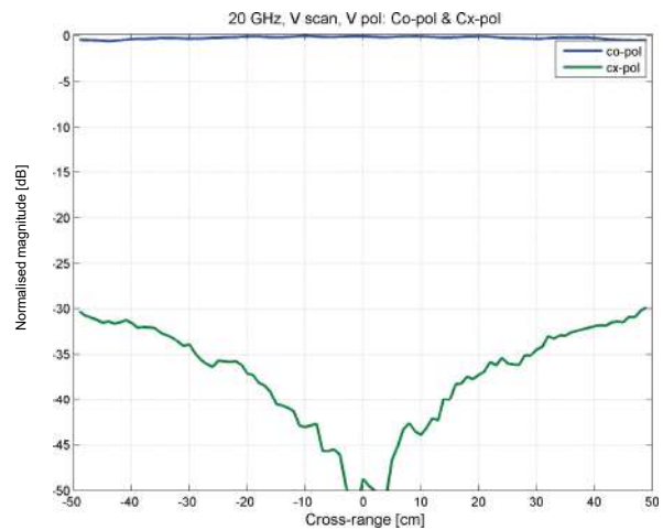
Quiet Zone Cross Polarisation
